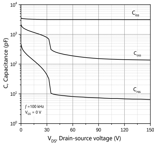
Figure 3. Typ. capacitances
