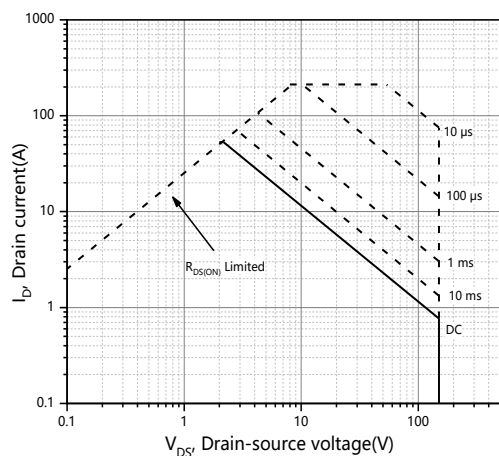
Figure 11. Safe operation area Tc=25°C
