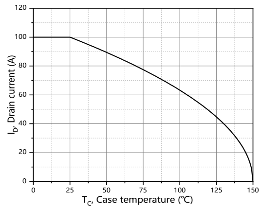
Figure 10. Drain current
