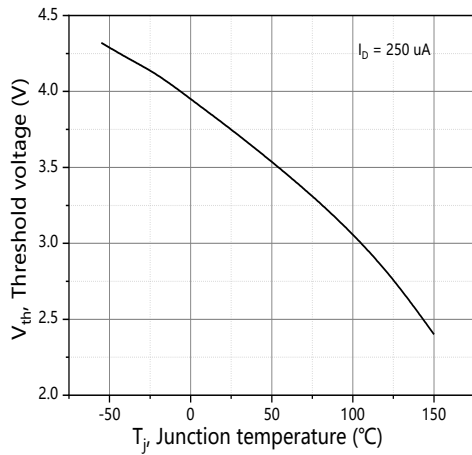
Figure 7. Threshold voltage
