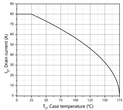
Figure 10. Drain current
