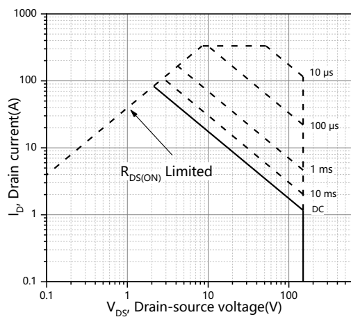
Figure 11. Safe operation area T_C=25\text{ }^{\circ}\text{C}
