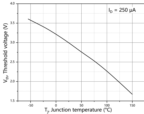
Figure 7. Threshold voltage
