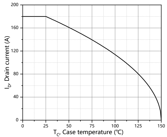
Figure 10. Drain current
