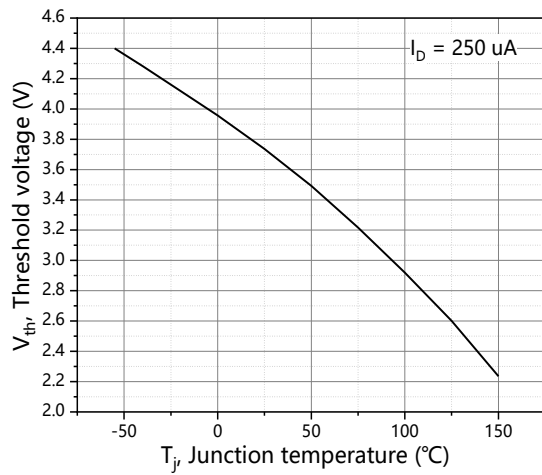
Figure 7. Threshold voltage
