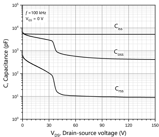
Figure 3. Typ. capacitances
