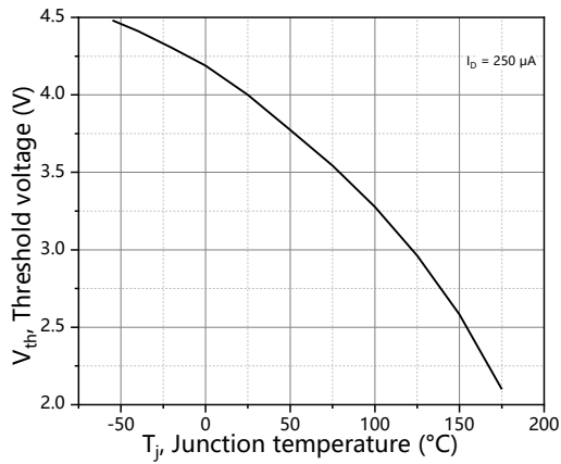
Figure 7. Threshold voltage
