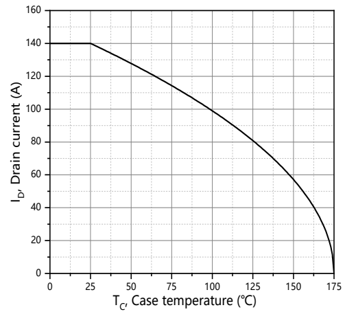
Figure 10. Drain current
