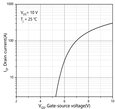
Figure 2. Typ. transfer characteristics
