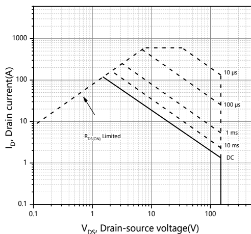
Figure 11. Safe operation area T_C=25^\circ C
