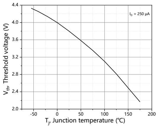
Figure 7. Threshold voltage
