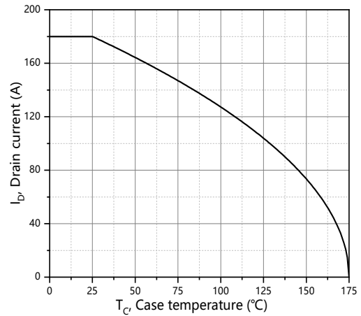
Figure 10. Drain current
