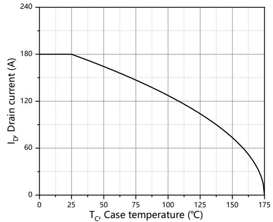
Figure 10. Drain current
