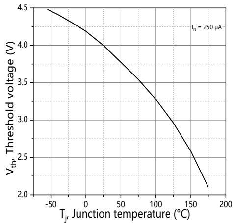
Figure 7. Threshold voltage
