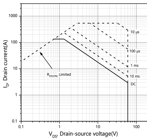
Figure 11. Safe operation area T_C=25\text{ }^{\circ}\text{C}
