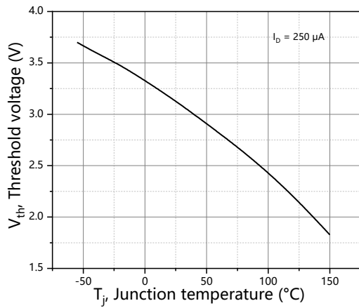
Figure 7. Threshold voltage
