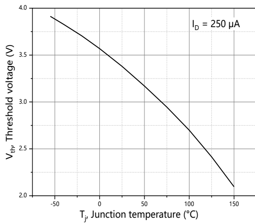
Figure 7. Threshold voltage
