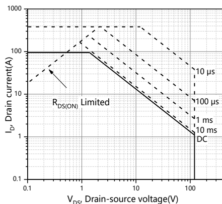
Figure 11. Safe operation area T_c=25\text{ }^{\circ}\text{C}
