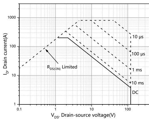
Figure 11. Safe operation area T_C=25^{\circ}\text{C}
