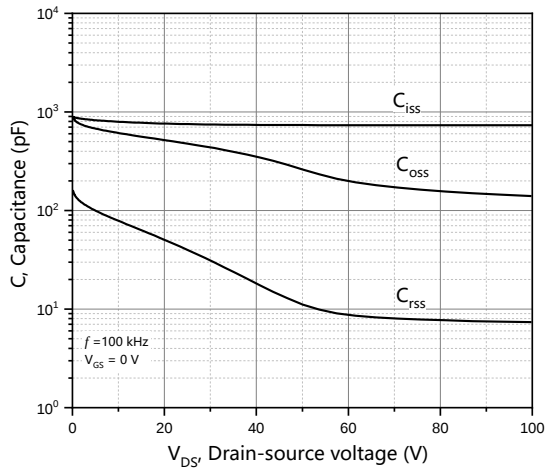
Figure 3. Typ. capacitances
