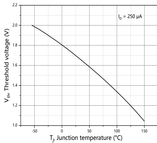
Figure 7. Threshold voltage
