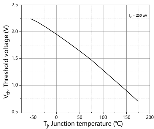
Figure 7. Threshold voltage
