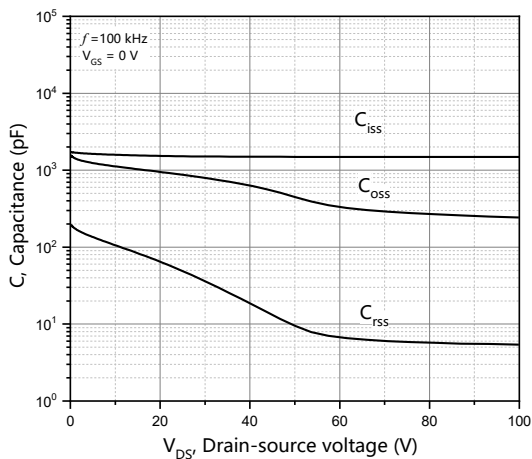
Figure 3. Typ. capacitances
