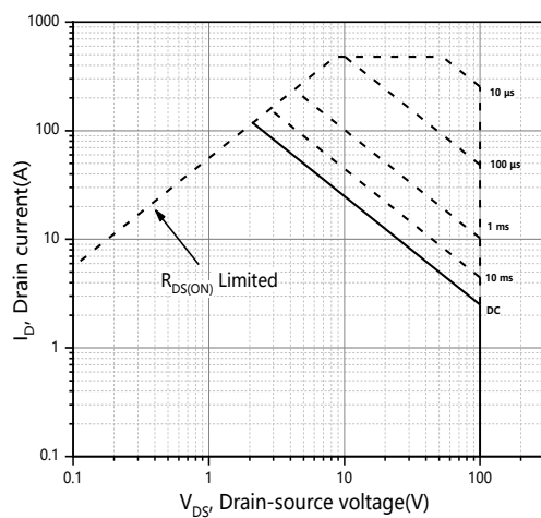
Figure 11. Safe operation area Tc=25°C
