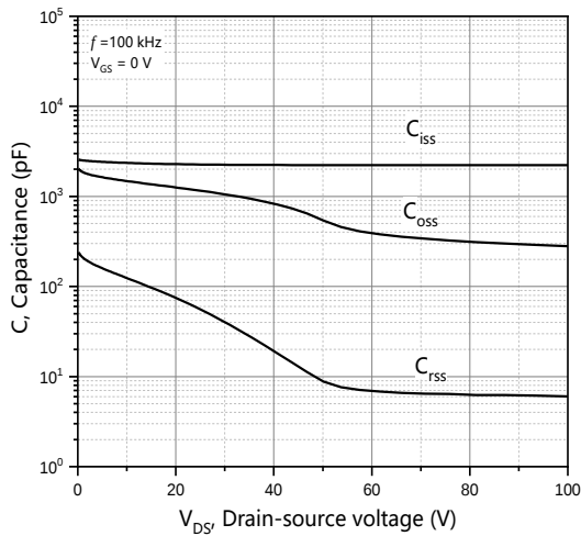
Figure 3. Typ. capacitances
