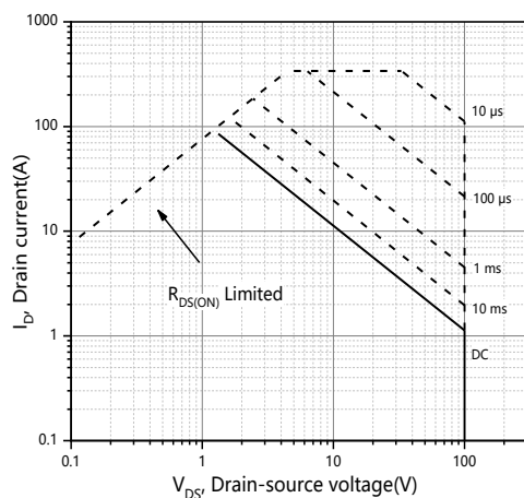
Figure 11. Safe operation area T_C = 25^\circ C
