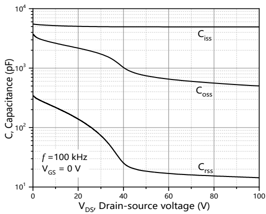
Figure 3. Typ. capacitances
