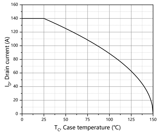
Figure 10. Drain current
