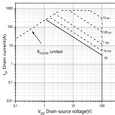
Figure 11. Safe operation area T_C=25^{\circ}\text{C}
