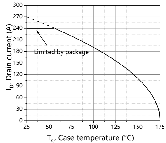
Figure 10. Drain current
