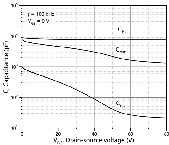
Figure 3. Typ. capacitances
