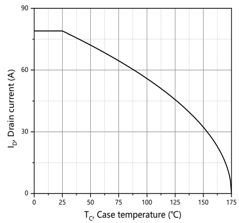
Figure 10. Drain current
