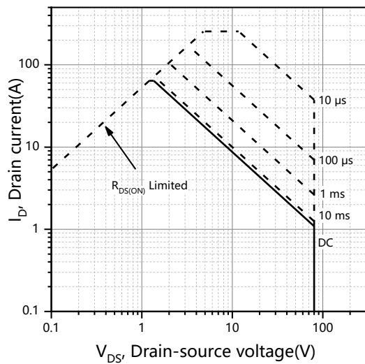
Figure 11. Safe operation area T_c=25\text{ }^{\circ}\text{C}
