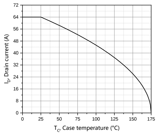
Figure 10. Drain current
