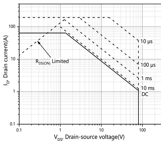
Figure 11. Safe operation area T_C=25 \text{ °C}
