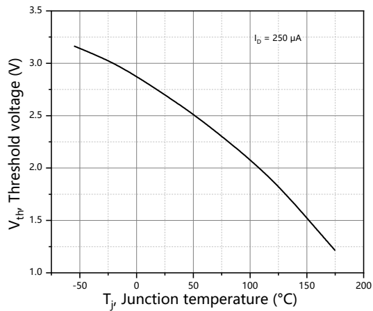
Figure 7. Threshold voltage
