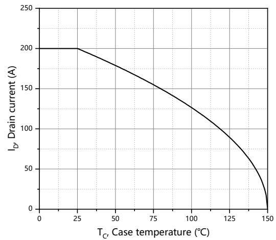
Figure 10. Drain current
