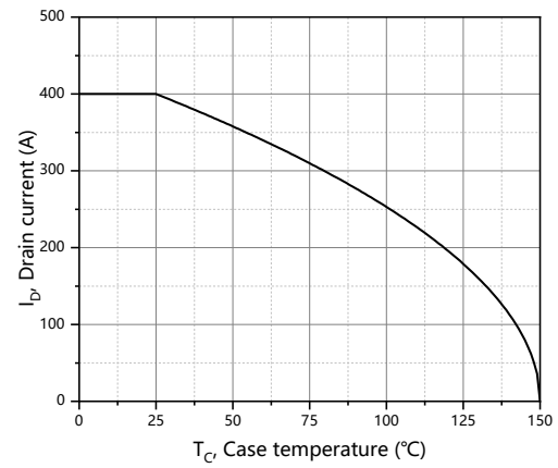
Figure 10. Drain current
