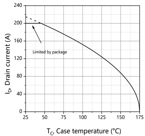
Figure 10. Drain current
