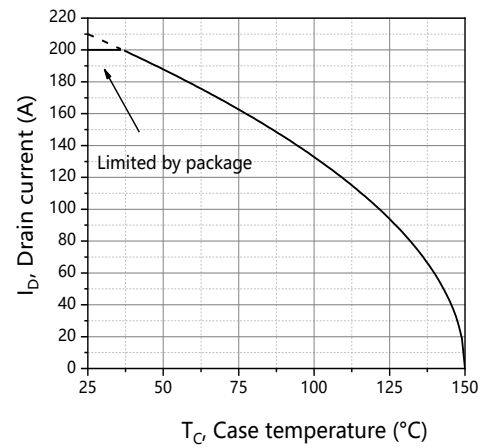
Figure 10. Drain current
