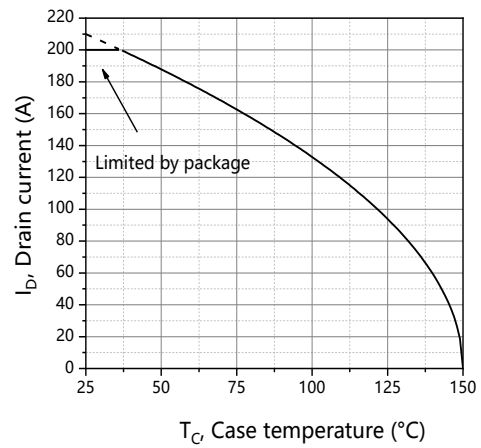
Figure 10. Drain current
