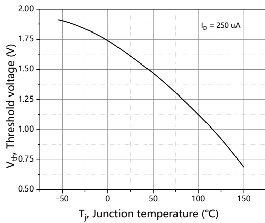
Figure 7. Threshold voltage
