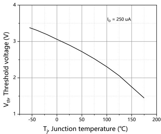
Figure 7. Threshold voltage
