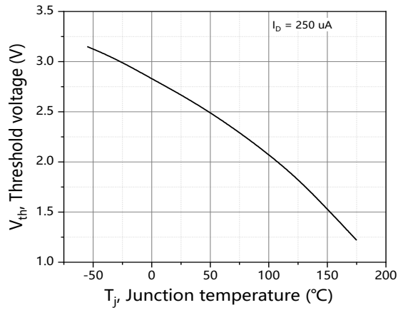
Figure 7. Threshold voltage
