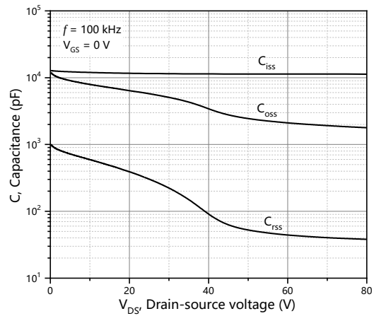
Figure 3. Typ. capacitances
