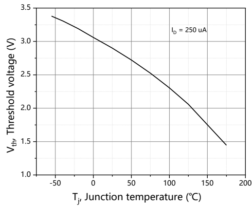
Figure 7. Threshold voltage
