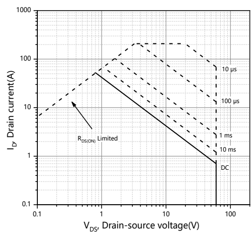
Figure 11. Safe operation area T_C=25^{\circ}\text{C}
