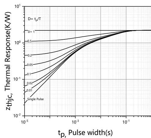
Figure 12. Max. transient thermal impedance
