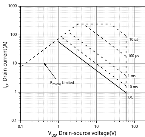
Figure 11. Safe operation area T_C=25\text{ }^{\circ}\text{C}
