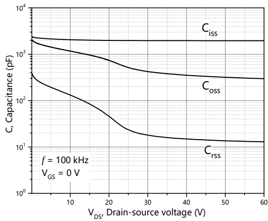
Figure 3. Typ. capacitances
