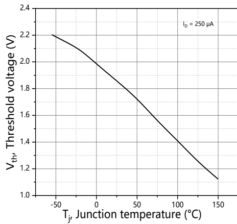
Figure 7. Threshold voltage
