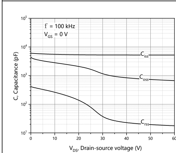
Figure 3. Typ. capacitances
