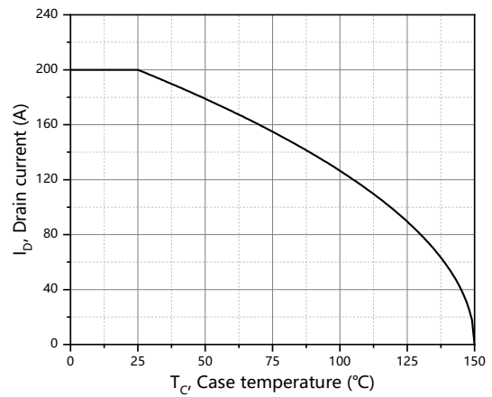
Figure 10. Drain current
